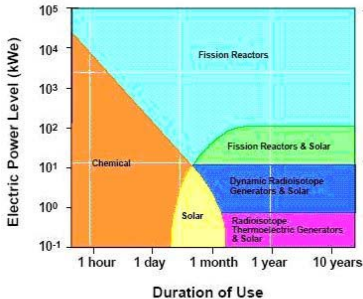
Figure 1 - Required Power Level versus Mission Duration for Space Applications 3
