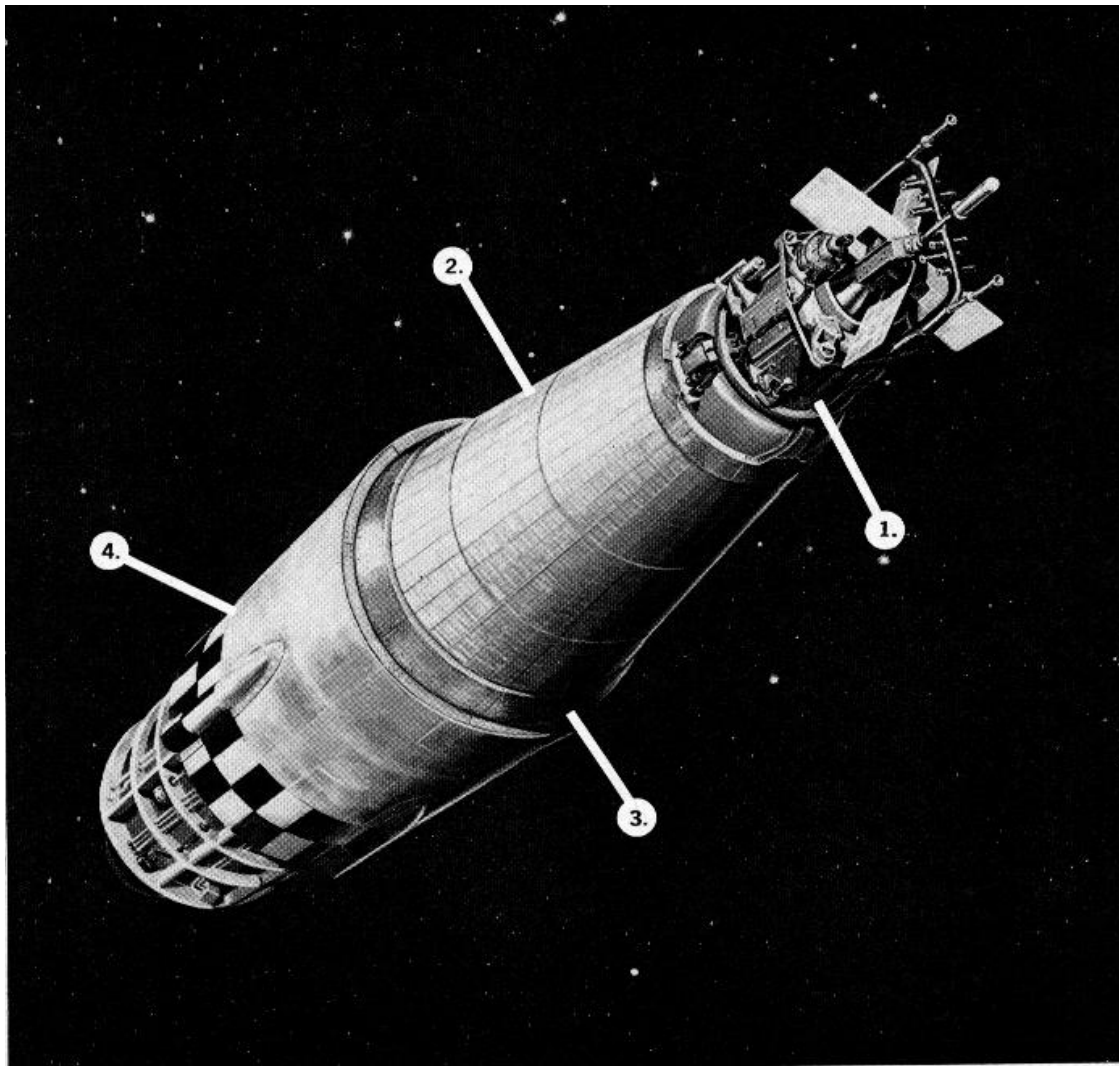
1. Nuclear reactor to produce heat 2. Thermoelectric units to convert heat into electricity 3. Instrumentation compartment 4. Agena vehicle
