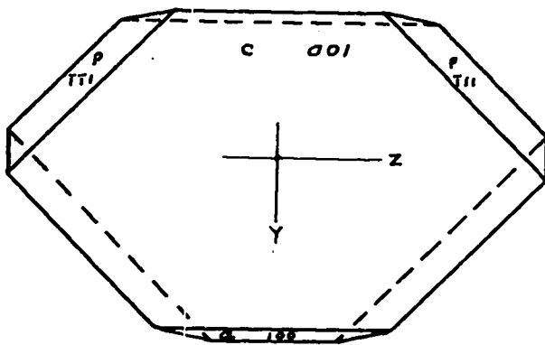
(b) Projection on C\ (001) .
