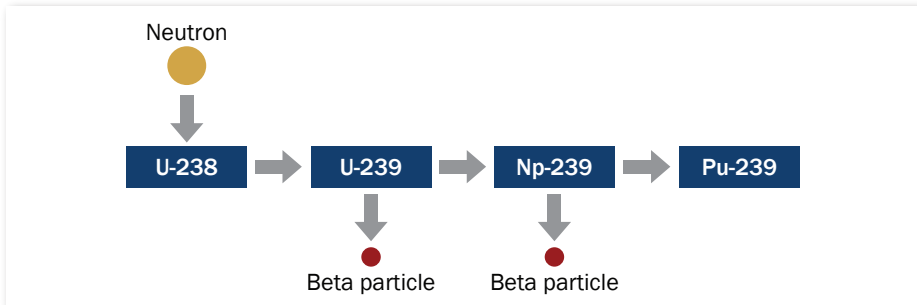
Figure 15.8 U-238 Neutron Capture and Transmutation to Plutonium
