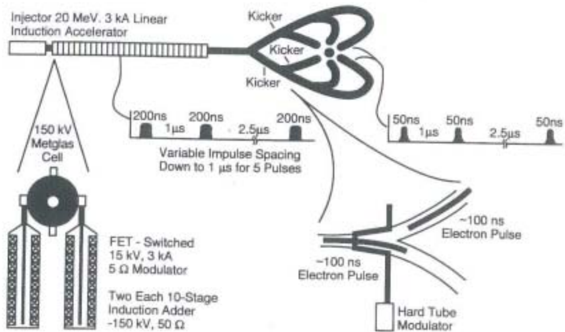
Figure 6-1. Design of the proposed advanced Hydro Test Facility (AHTF) illustrating multiple time-dependent image capability.
