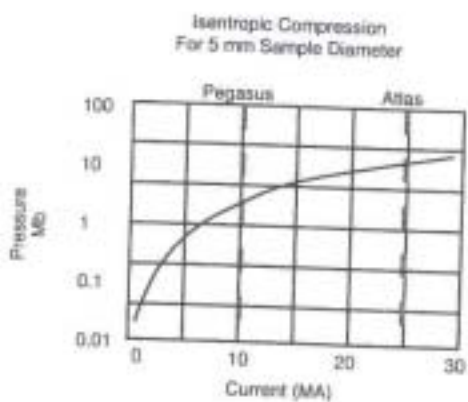
Figure 9-3. Atlas will be used for hydronamic experiments.
