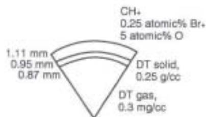
Capsule detail
